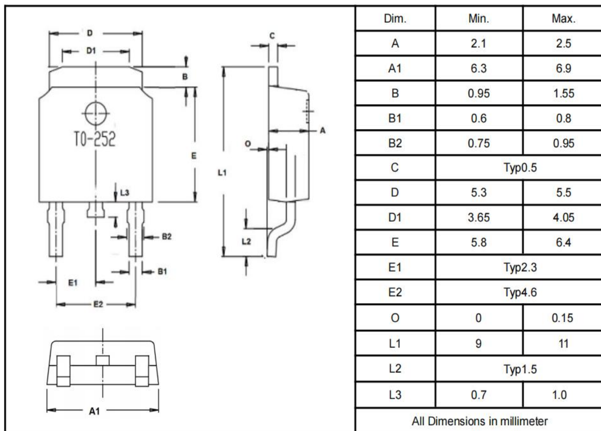
TO-252
