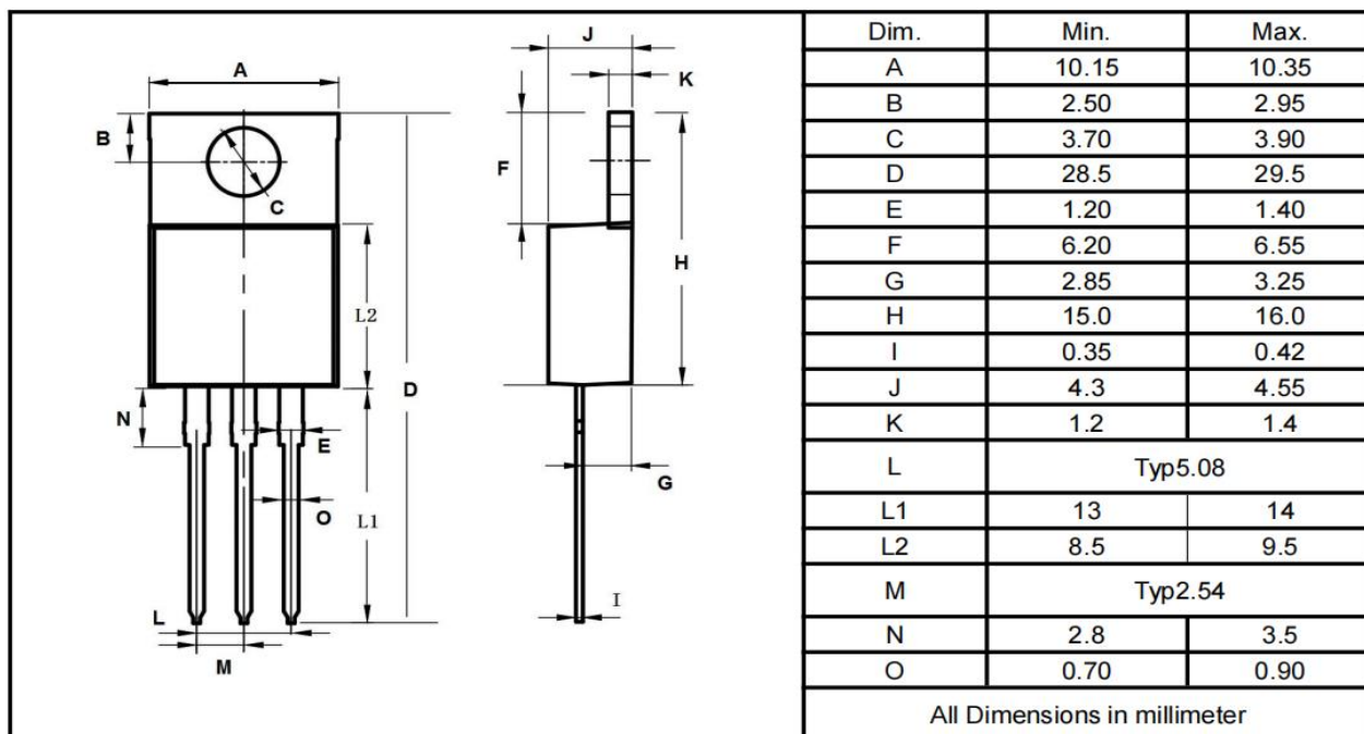
TO-220AB
