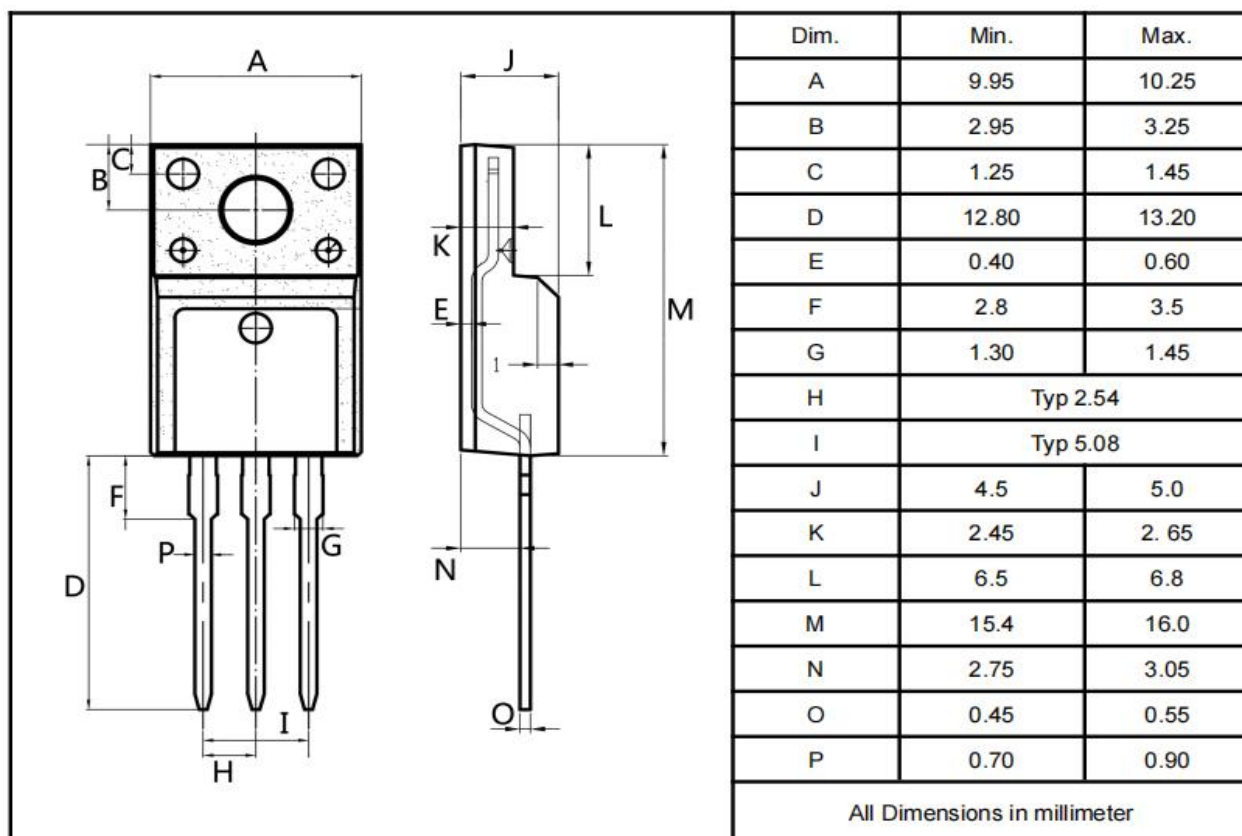
TO-220F
