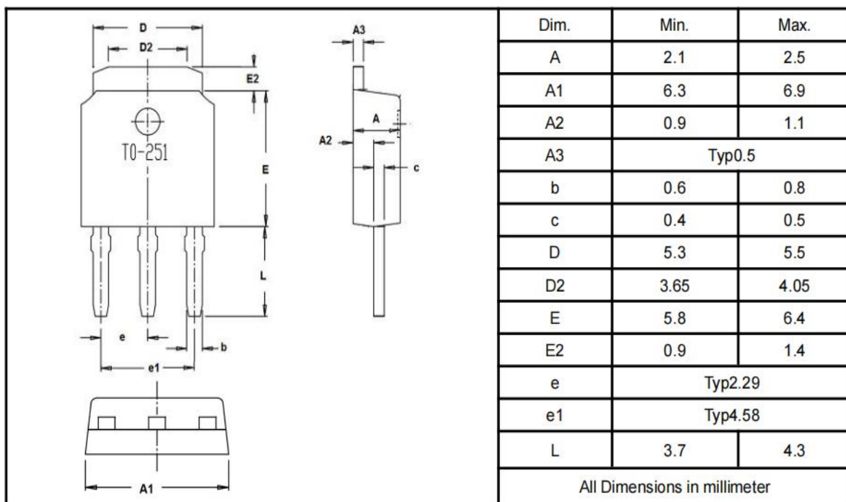
TO-251
